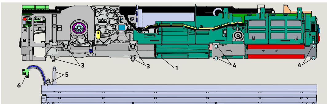
Fig. 8.2.2 Mounting plate removed from ED50LE operator
