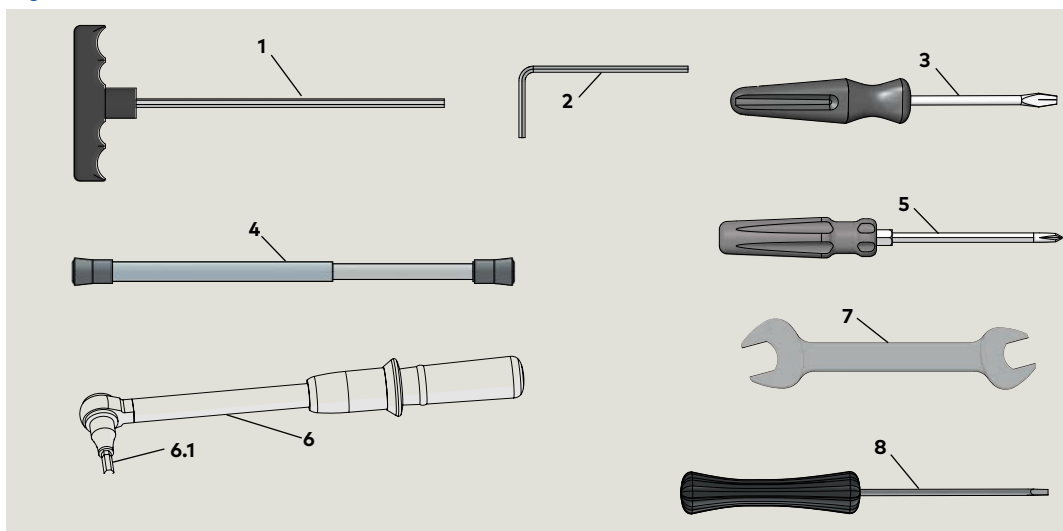
Fig. 6.1.1 Recommended tools
