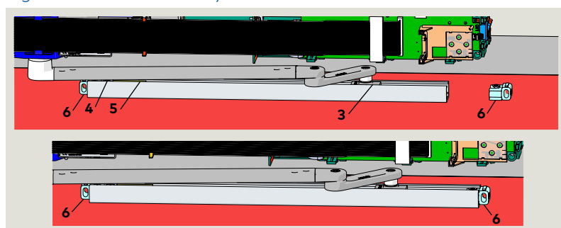
Fig. 10.8.3 Track assembly installed onto slide shoe
