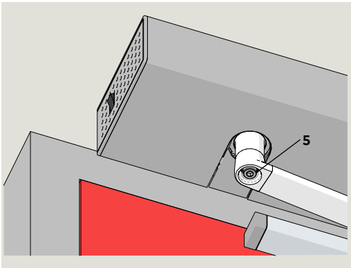
Fig. 15.2.3 Pivot pin M8 socket head
