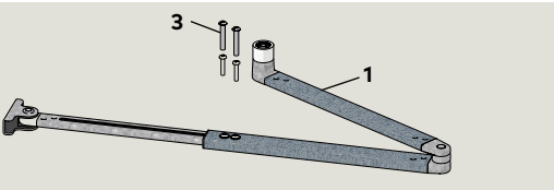
Fig. 2.7.2 Deep pull arm kit, HK4709-12X
