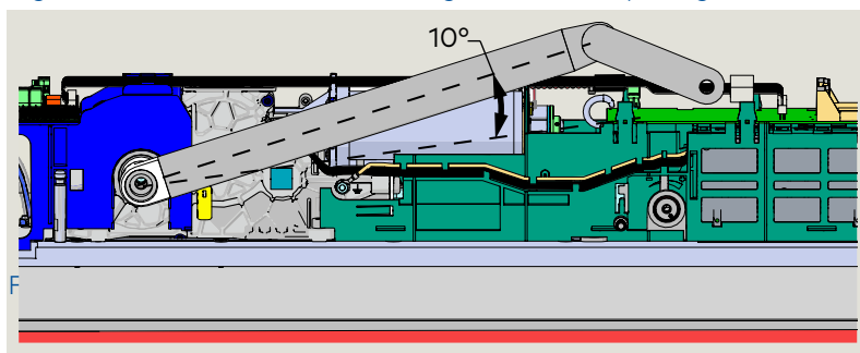
Fig. 10.7.3 Remove drive arm from ED50LE spindle
