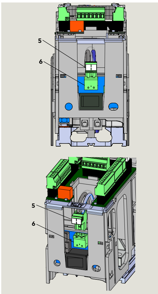
Fig. 8.2.2 Mounting plate removed from ED50LE operator
