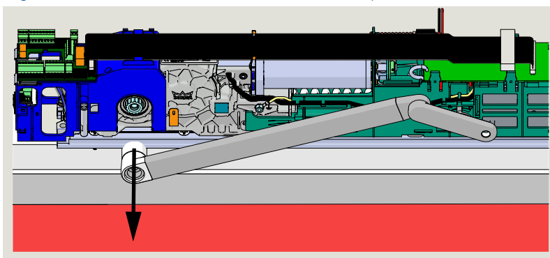
Fig. 10.7.4 Install drive arm and extension onto ED50LE spindle
