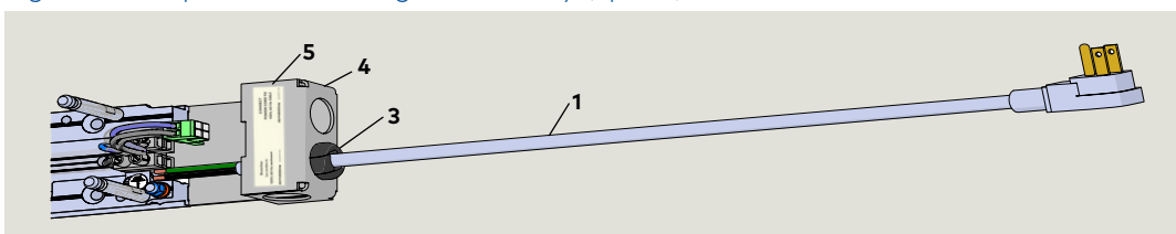
Fig. 8.3.7 PC power cord wiring kit assembly (option)
